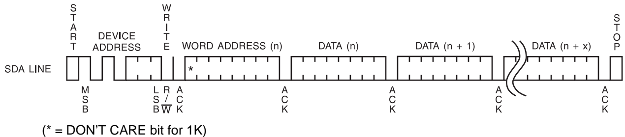
Figure 3. Page Write
